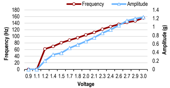
Figure 3. Measured frequency and amplitude of an ERM vibromotor mounted on a user’s wrist as applied voltage changes. Graph adapted from our prior work [18].
