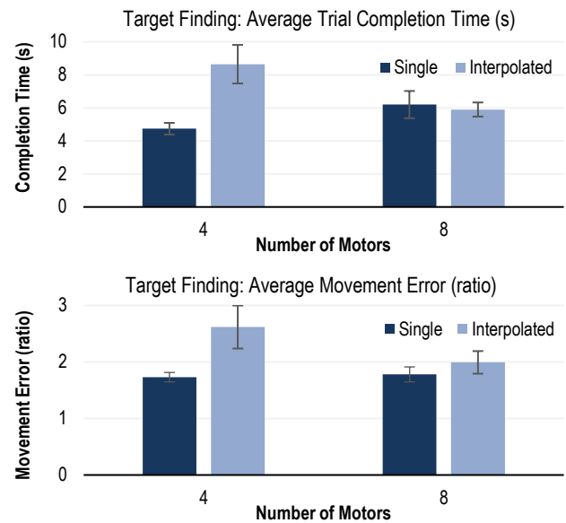
Figure 7. Average trial completion time and movement error for the target-finding task in Study 1, showing interpolated feedback is less accurate than single-motor feedback. Error bars show standard standard error. ( N = 13 )
