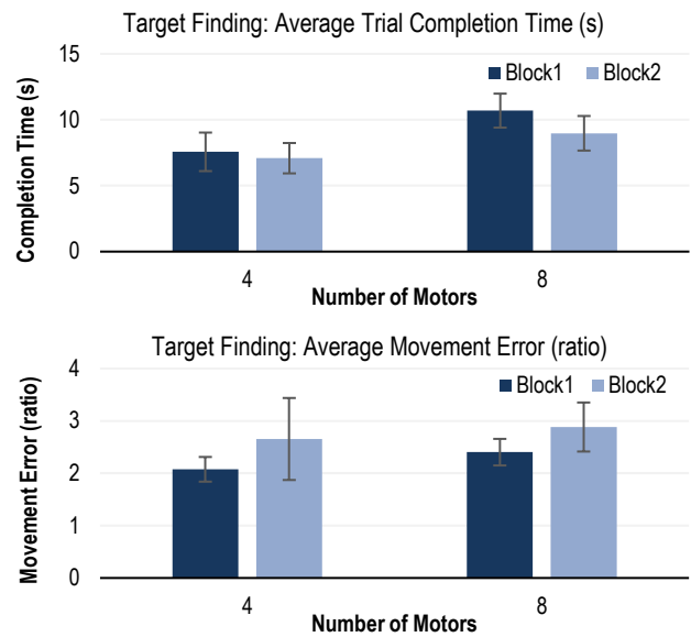
Figure 10. Trial completion time and movement error for the target-finding task in Study 2. The 4-motor wristband was faster and more accurate than the 8-motor wristband. Error bars are standard error. ( N = 14 )
