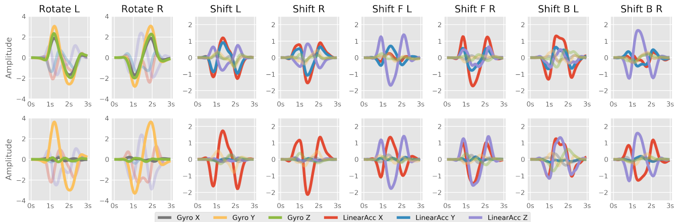
Figure 6: IMU signals of the eight waist gestures collected by a phone put in the right front trouser pocket. The top row shows the original data with a Butterworth low-pass filter at 2 Hz. The bottom row shows the data after transformation. Gyroscope/linear accelerometer signals are highlighted with higher opacity for rotating/shifting gestures respectively.
